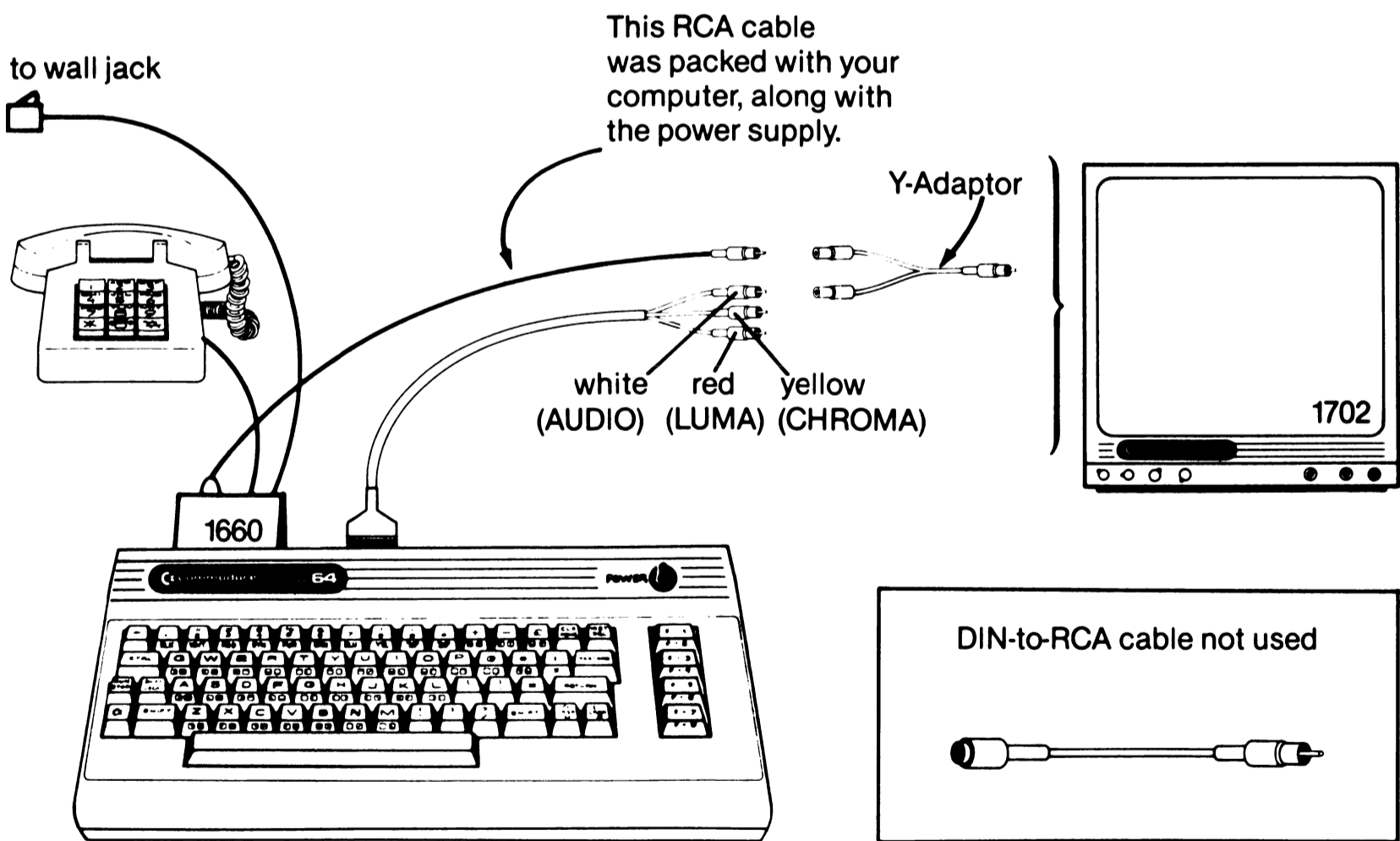
FIGURE 2-1. CONNECTION DIAGRAM
